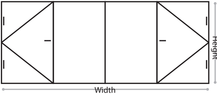
4 Panel (Side Hung Left : Fixed : Fixed : Side Hung Right)
